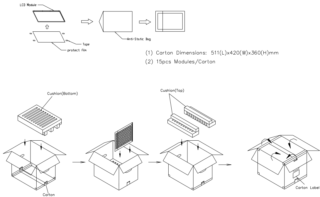
Figure. 9-1 Packing method
